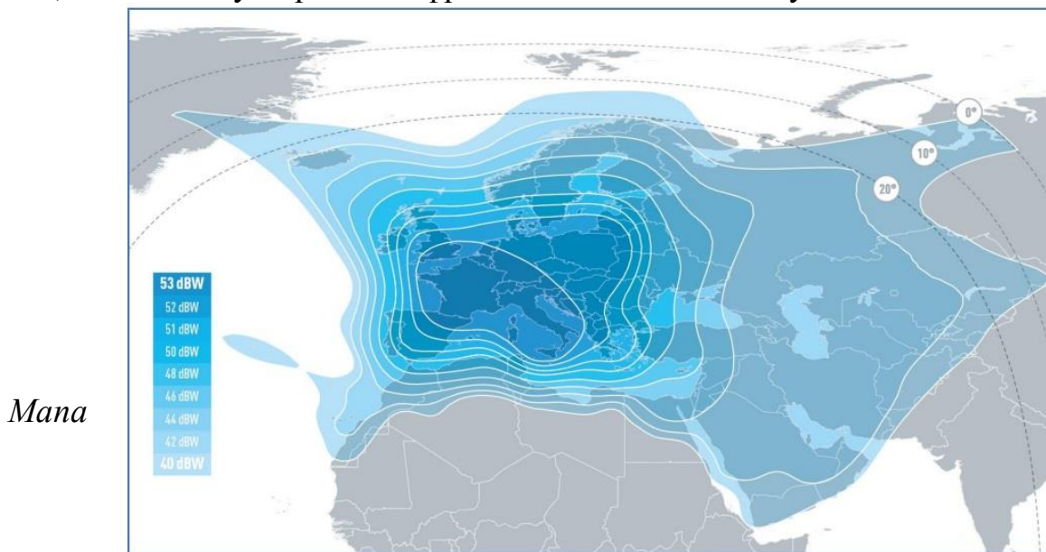
HOTBIRD™ 13G Ku Band Widebeam Downlink Coverage in dBW
